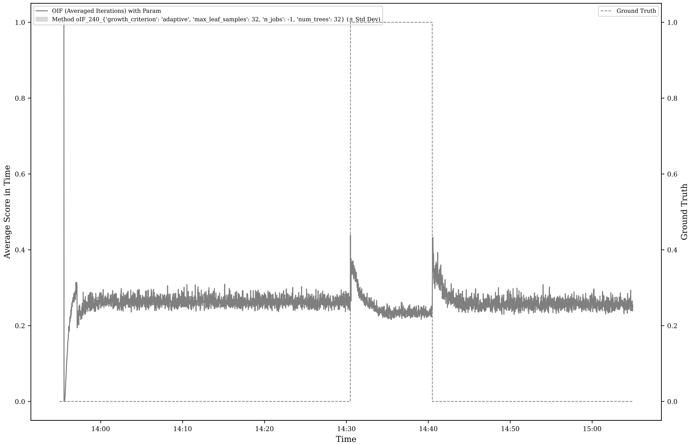
Method OIF Score for Scenario A6
